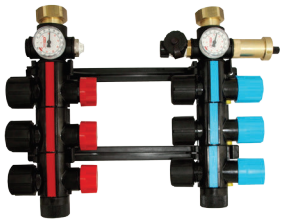
HEATLINK MANIFOLD
